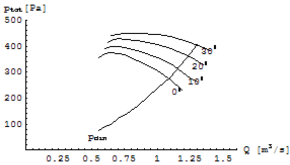
DV70N 0 3.55 P=0.55 kW at 0° n=1360 min -1
