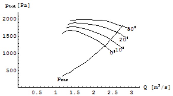
DV70N 0 3.55 P=4 kW at 0° n=2870 min -1
