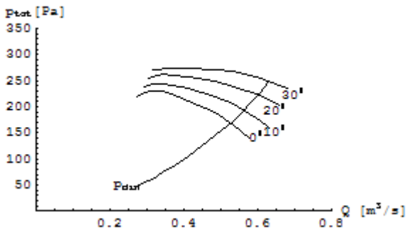
DV70N 0 2.8 P=0.25 kW at 0° n=1350 min -1
