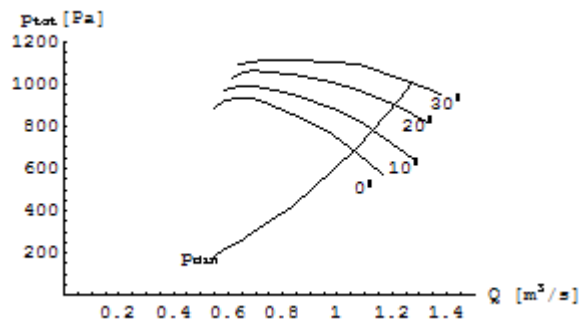
DV70N 0 2.8 P=1.1 kW at 0° n=2800 min -1
