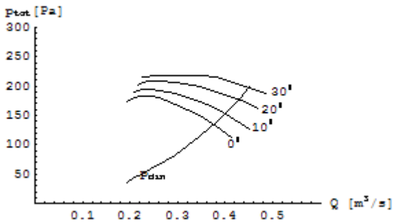
DV70N 0 2.5 P=0.12 kW at 0° n=1350 min -1
