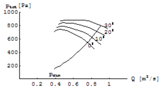
DV70N 0 2.5 P=0.55 kW at 0° n=2720 min -1
